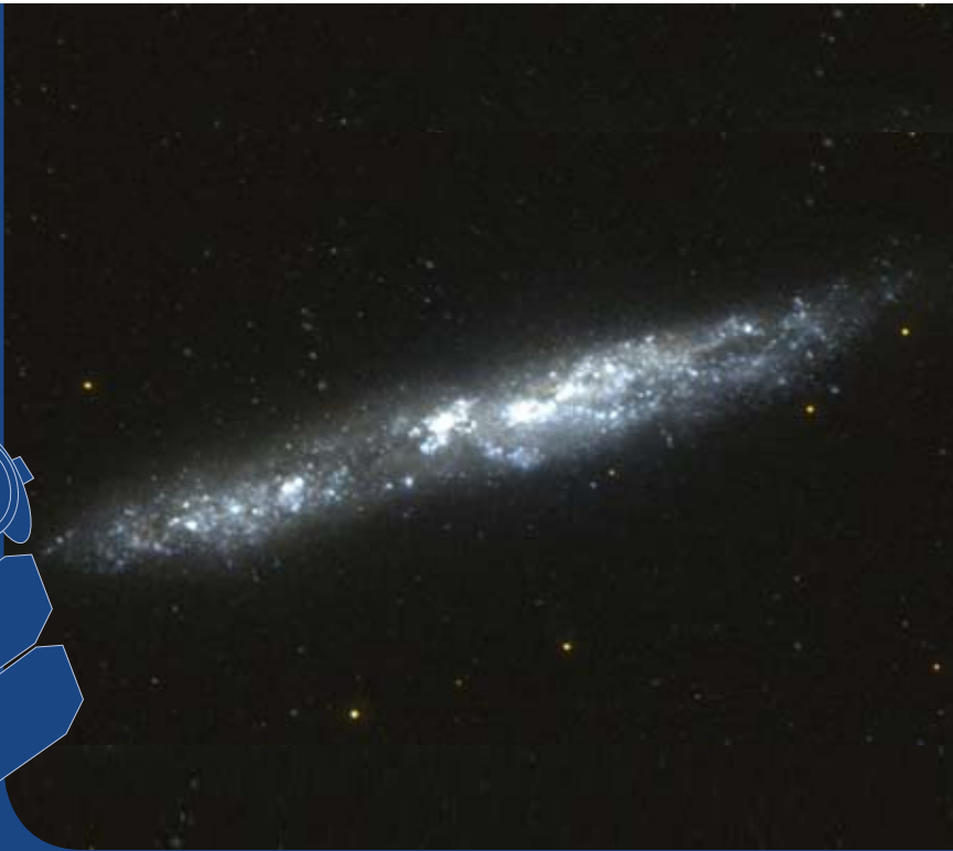
Galaxy NGC 55
